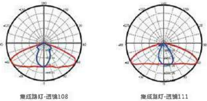
配光曲线图 Light Distribution Curve
